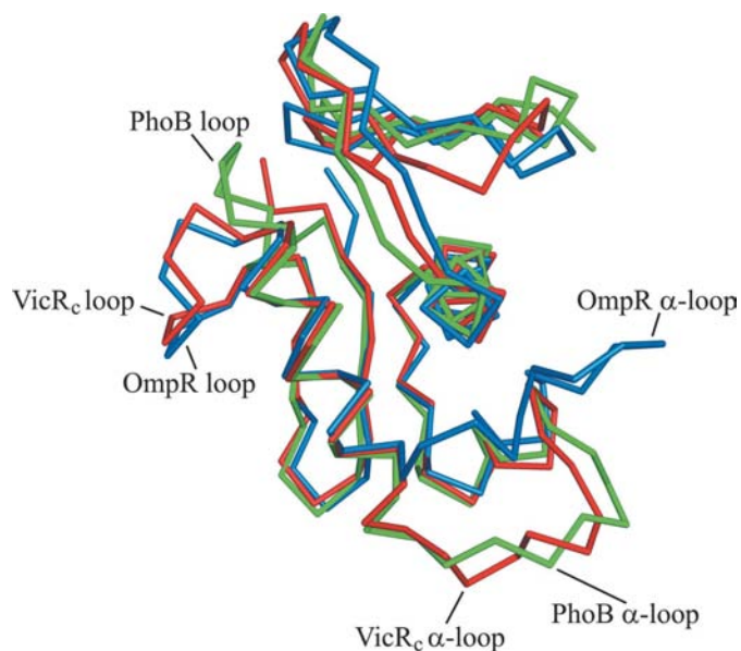
Figure 2 Structural comparison of the C \alpha backbones of VicR c (red), PhoB (green) and OmpR (blue). The \alpha -loops and the loops linking \alpha 3 to the C-terminal \beta -hairpin are labelled.
